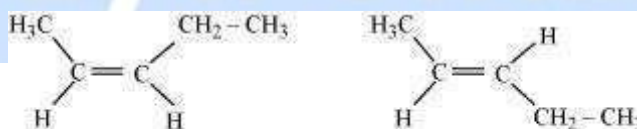
Cis - isomer
